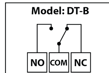
Wiring Detail
