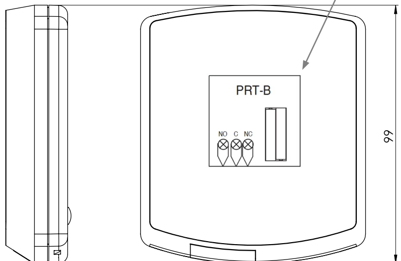
Wiring Detail
