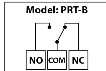
Wiring Detail
